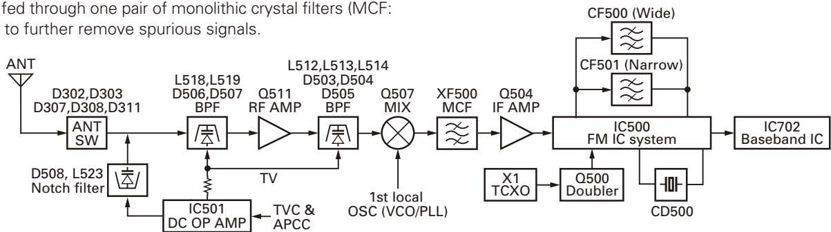
Fig. 2 Receiver System
