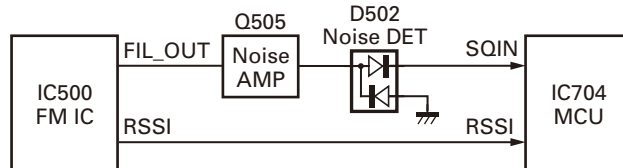
Fig. 5 Squelch circuit
