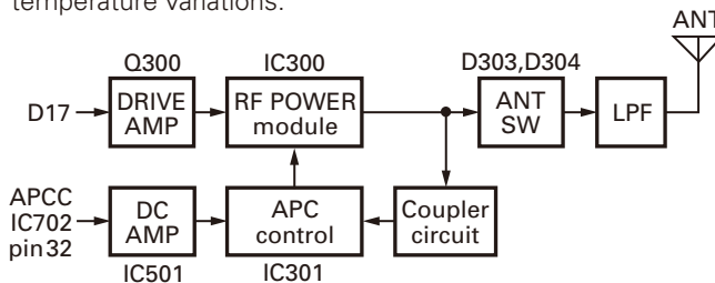
Fig. 7 APC circuit
