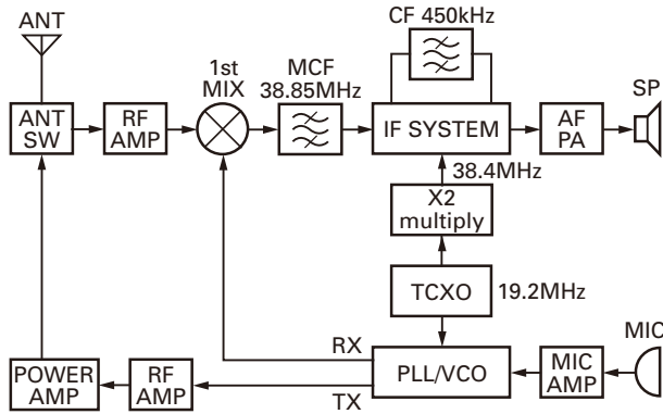
Fig. 1 Frequency configuration
