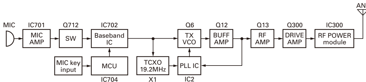
Fig. 6 Transmitter system
